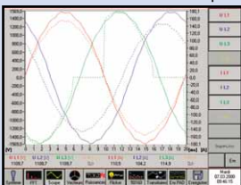
Oscilloscope 8 traces
